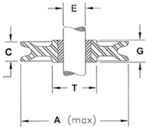
BRONZE BUSHED SHEAVE
