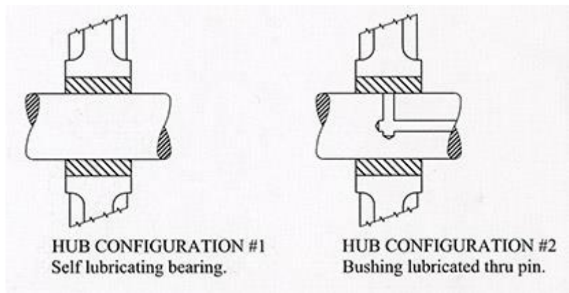
BRONZE BUSHED SHEAVE
